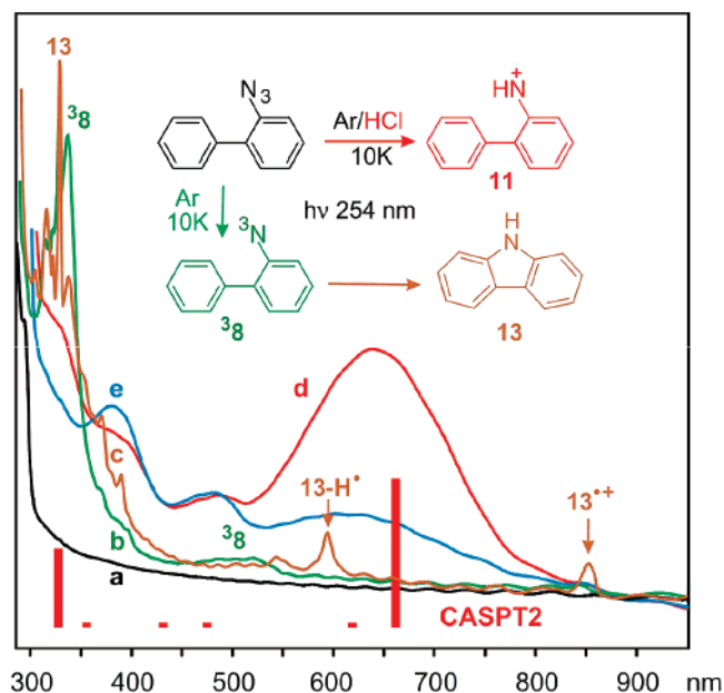
Figure 5. (a) UV-vis spectrum of o -biphenyl azide 7 in Ar; (b) after short bleaching at 254 nm; (c) after longer bleaching at 254 nm; (d) after bleaching at 254 nm in the presence of 30% HCl in Ar; (e) after subsequent bleaching of 11 at \lambda > 590 nm.
