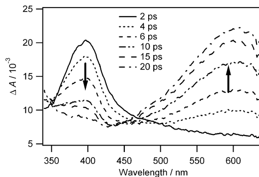
Figure 4. Transient spectra produced by ultrafast photolysis of o -biphenyl azide 7 in 88% formic acid. The spectra were generated by ultrafast LFP (270 nm) with a time window of 2–20 ps.
