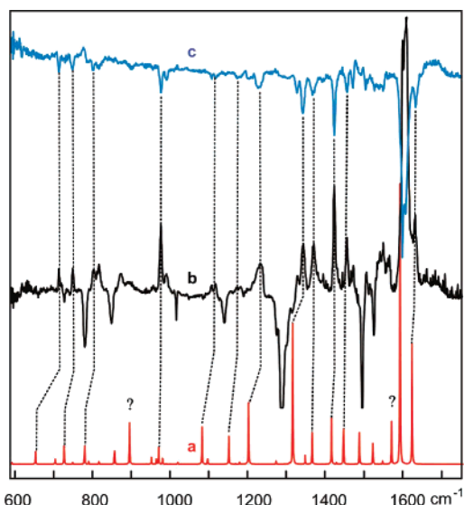
Figure 3. (a) IR spectrum of 6 calculated by B3LYP/6-31G*; (b) IR spectrum produced by bleaching of p -biphenyl azide 4 in Ar/HCl at 254 nm (negative peaks) and formation of the nitrenium cation 6 (positive peaks); (c) bleaching of 6 by irradiation at \lambda > 590 nm (negative peaks).
